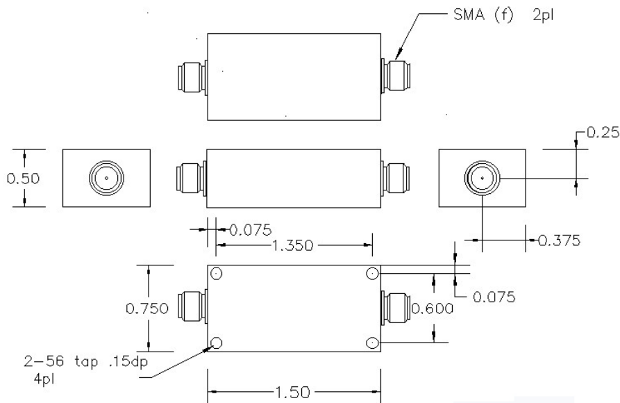
Outline Drawing 986215
