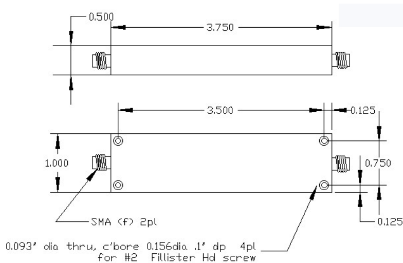
Outline Drawing 986187
